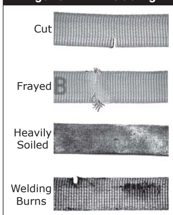
Figure 27 - Webbing
