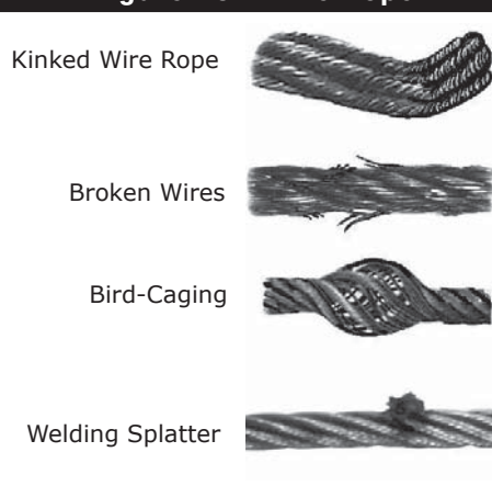
Figure 28 - Wire Rope
