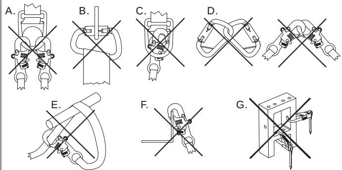
Figure 6 – Inappropriate Connections
