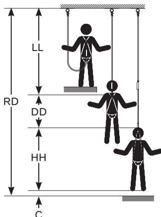
Figure 2 – Fall Clearance
