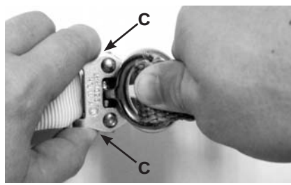
Figure 12 – Failed Connection
